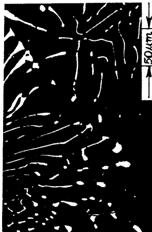
MC TYPE CARBIDES IN STEEL C11V FIG. 6
